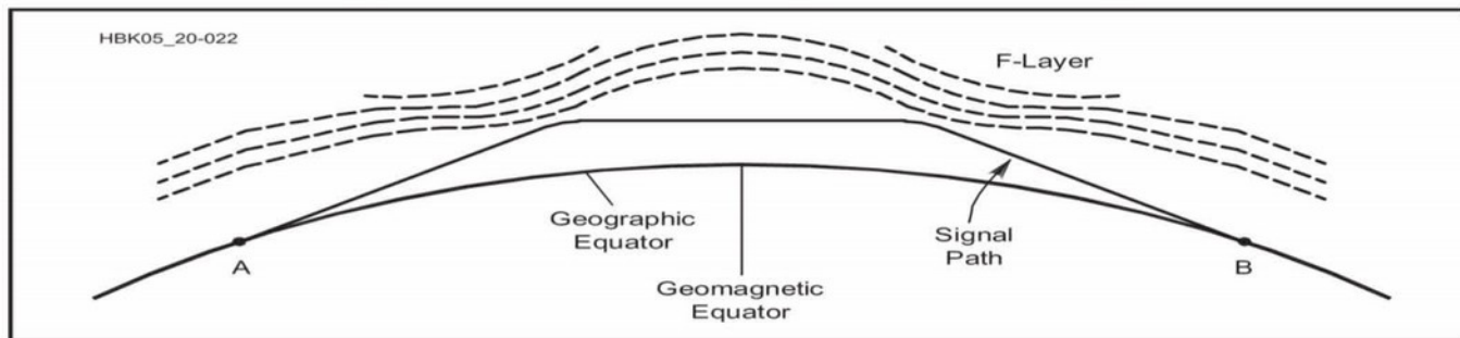
Fig 19.22 — Cross-section of a transequatorial signal path, showing the effects of ionospheric bulging and a double refraction above the normal MUF.
